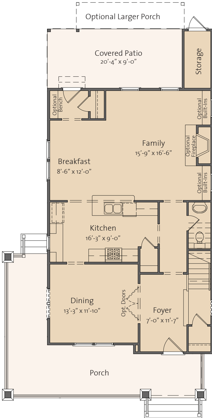
Foxworth F First Floor Plan
